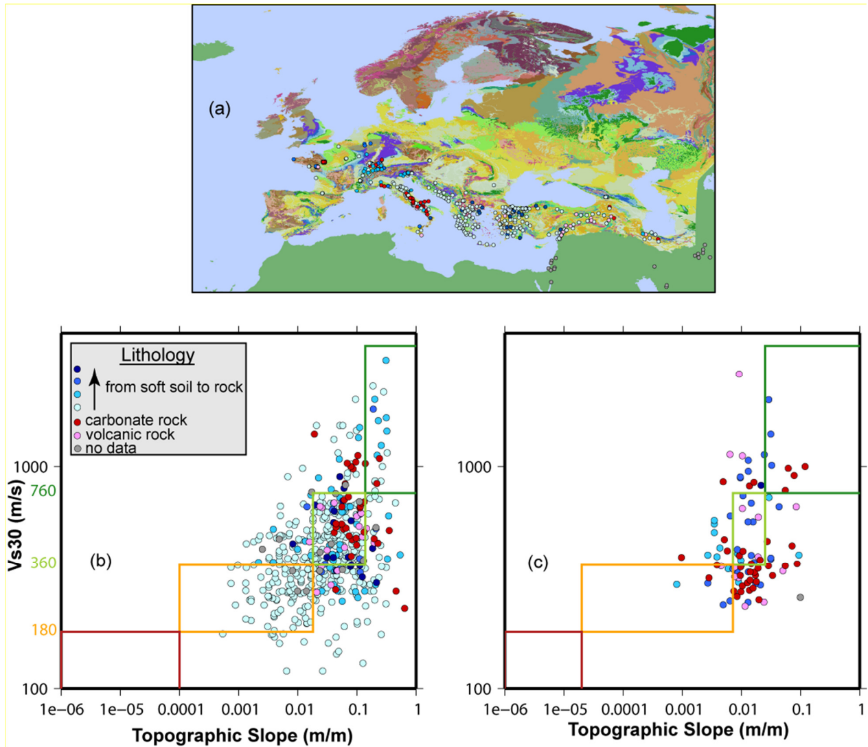
Figure 4: European geological map, distribution of V_{s30} -slope pairs for active and stable regions used in this study and the site class-slope correlations proposed by Wald and Allen (2007) as colored boxes.
