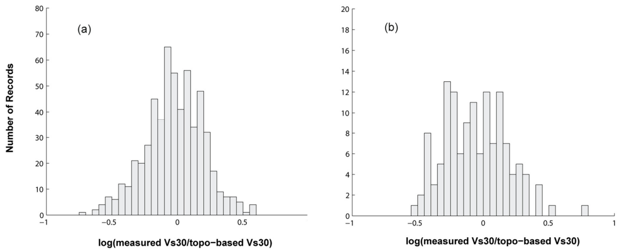
Figure 6: Histograms indicating logarithmic differences of measured V_{S30} values compared to those estimated by the approach of Wald and Allen (2007). For active regions (a) the bias is -0.024 and the standard deviation is 0.221 and for stable regions (b) the bias is -0.056 and the standard deviation is 0.241 .
