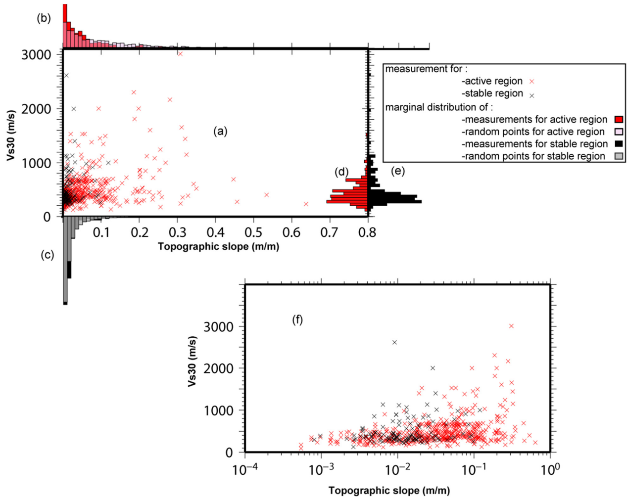
Figure 3: Distribution of V_{s30} -slope pairs used in this study (a). (b) and (c): marginal distributions of the slopes respectively for active and stable regions (including the true distribution obtained from 10 000 random locations distributed throughout Europe). (d) and (e): marginal distribution of V_{s30} values respectively for active and stable regions. (f) : same as (a) but with a logarithmic slope axis.
